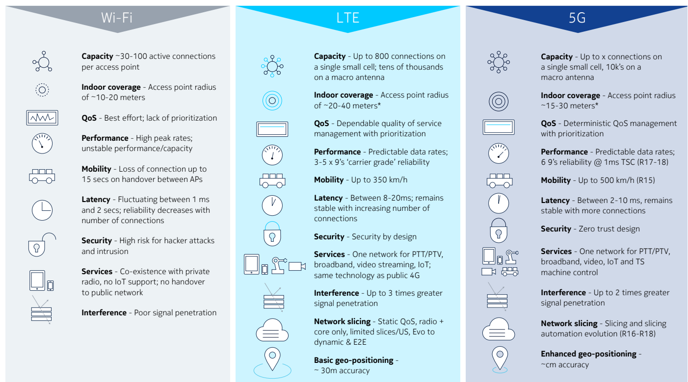
Figure 2. Comparison of Wi-Fi and LTE/5G
