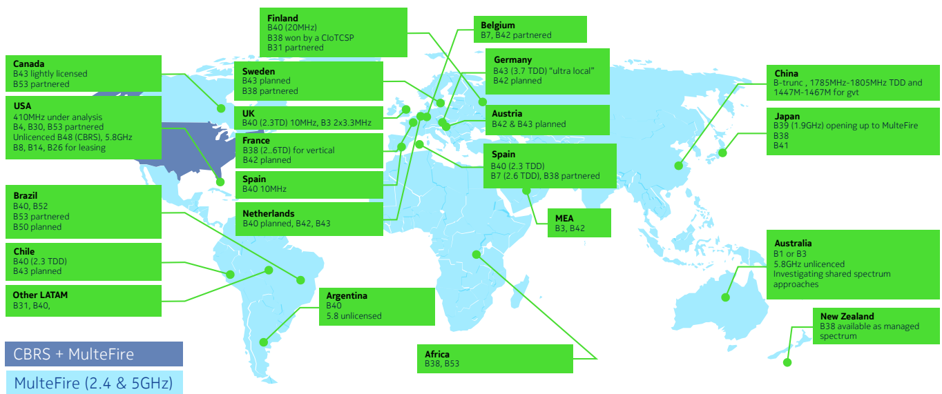
Figure 4. Private wireless spectrum options (LTE)
