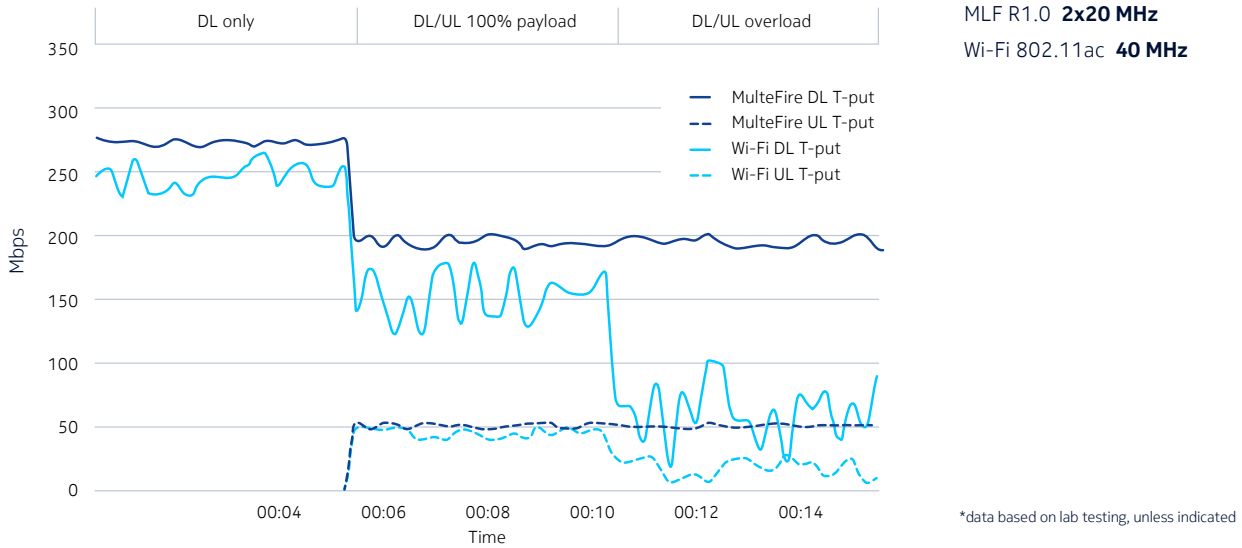
Figure 7. Comparison of throughput stability under load of 4.9G/LTE vs. Wi-Fi
