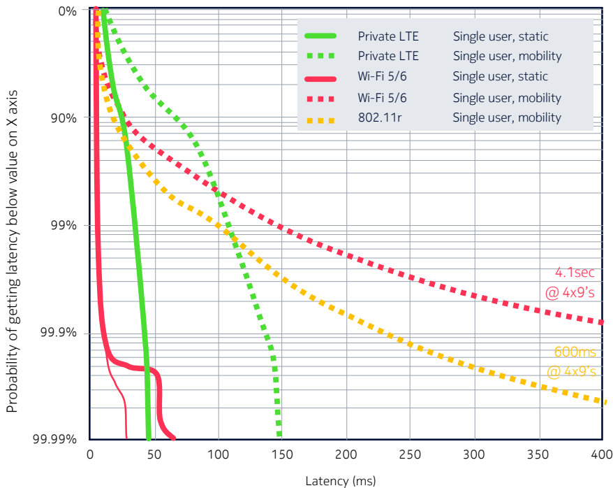
Figure 8. Comparison of LTE and Wi-Fi latencies for mobile devices.
