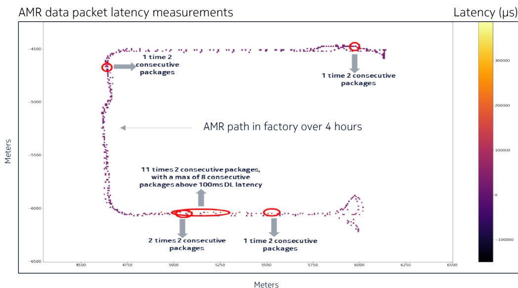
Figure 5. Benchmark of AIV communications over four hours
