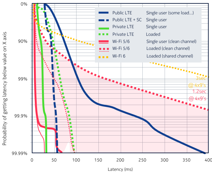
Figure 6. Latency measures for Wi-Fi vs. public and private LTE
